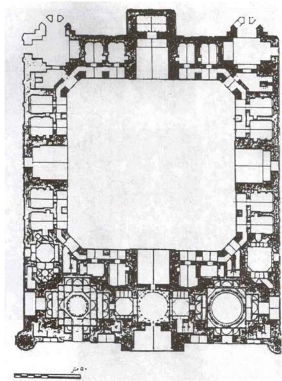
19. Khargerd, plan of Ghiasieh School, 1442-1445
